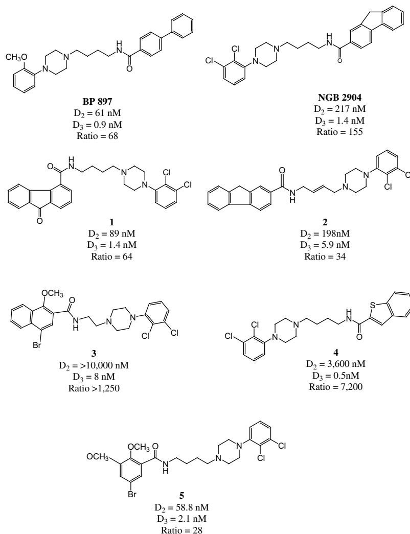
Figure 1. Structures of D 3 -selective benzamide analogs reported in the literature.
